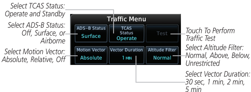
ADS-B Traffic Menu
