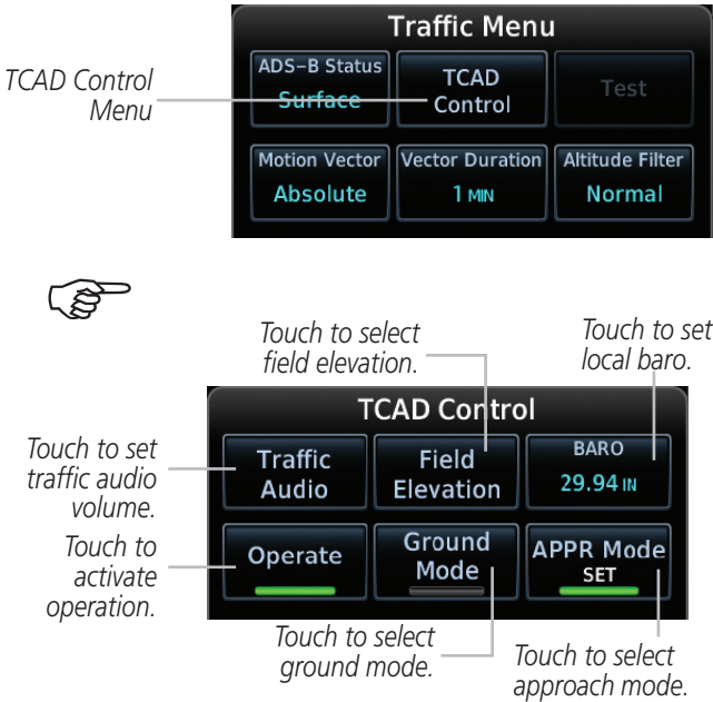
TCAD Traffic and Control Menu Control
